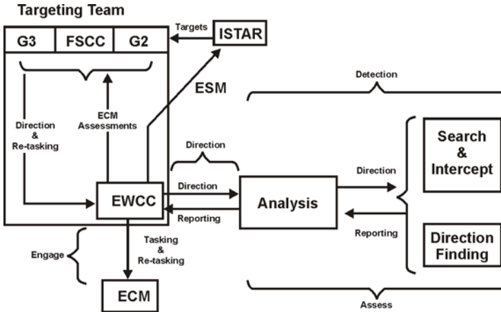
Figure 4-3: ECM process
