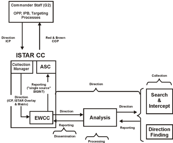
Figure 4-2: ESM Process
